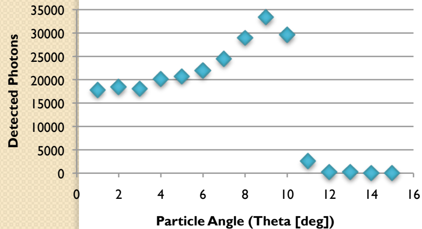
Hits vs. Particle Angle
