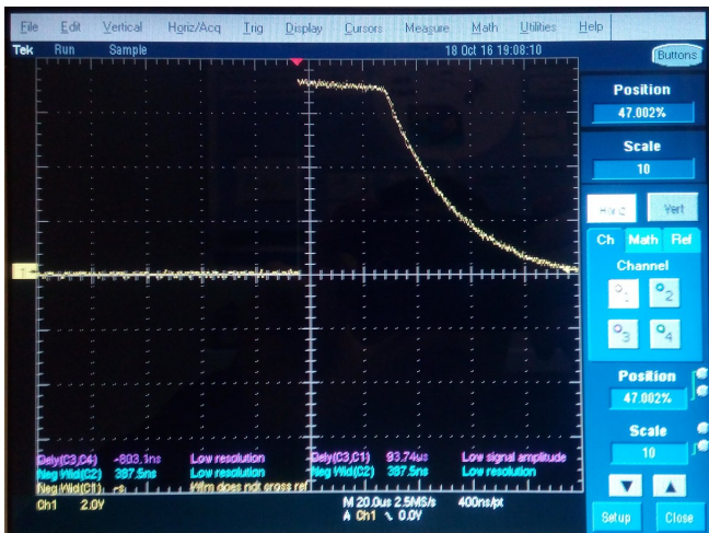
Figure: LED+PA+70V
