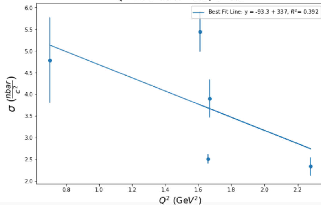
Q^2 vs \sigma at W=2.2, t=0.2
