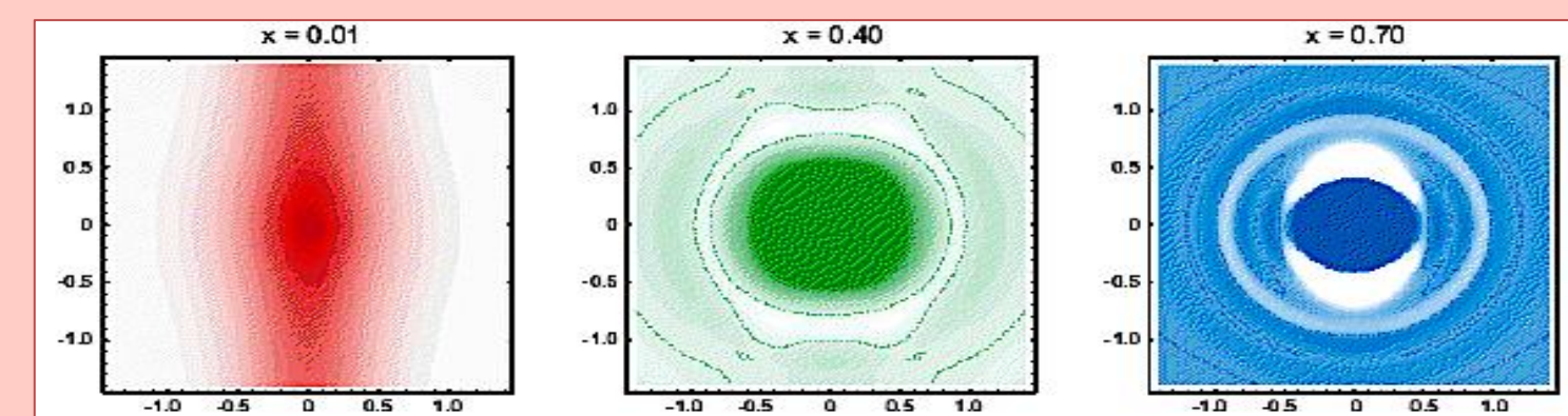
Pictures show transverse plane for different quark momentum fractions x
