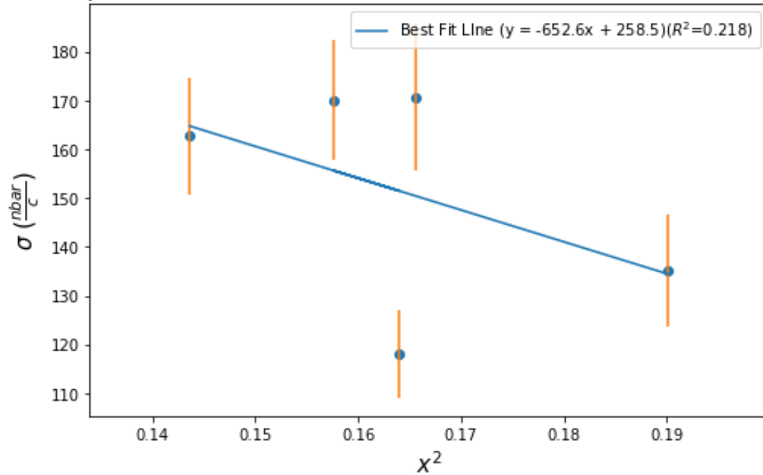
x^2 Dependence at Q^2=1.6 , W=2.2 , t=0.5-0.6 , x=0.3-0.5
