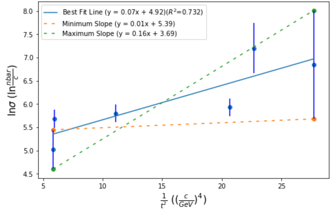
\frac{1}{t^2} Dependence at Q^2=1.6 , W=2.2 , t=0.2 , x=0.1-0.2
